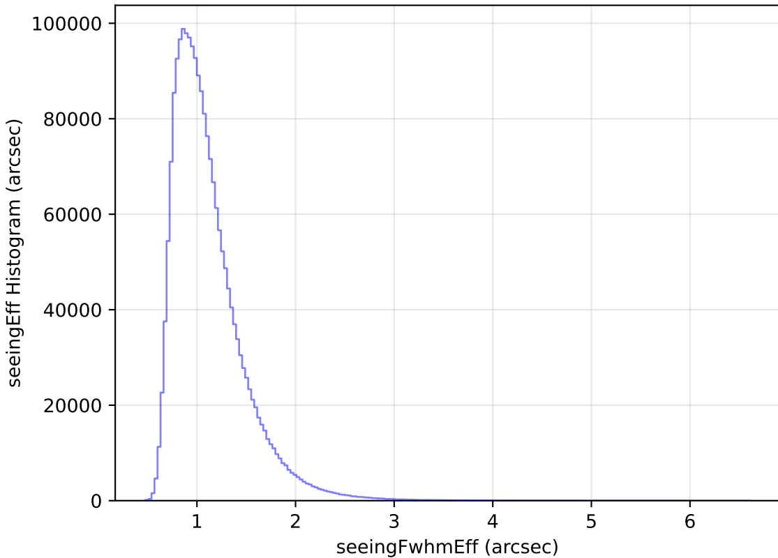
too_elab_heavy_r32_d2_griz_v3.4_10yrs WFD all bands: seeingEff Histogram
