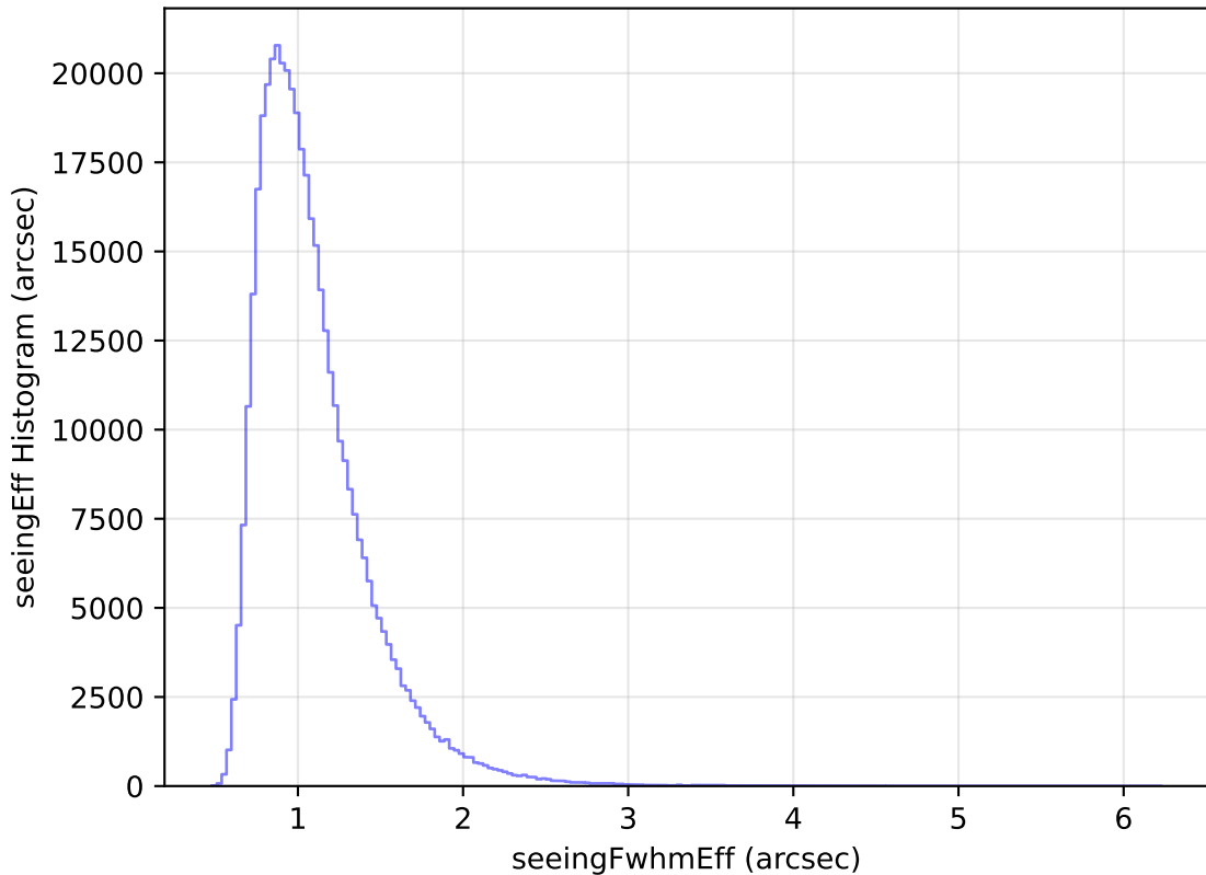
too_elab_heavy_r32_d2_griz_v3.4_10yrs All sky z band: seeingEff Histogram
