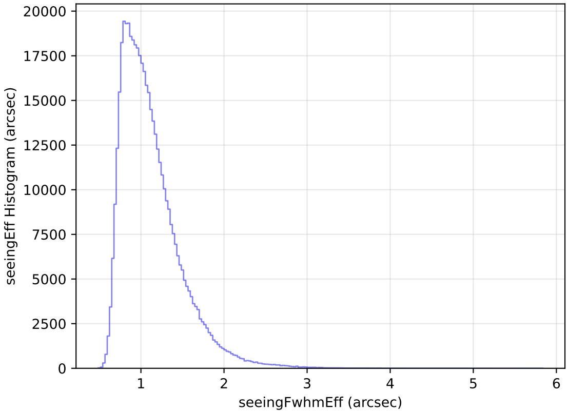
too_elab_heavy_r32_d2_griz_v3.4_10yrs All sky r band: seeingEff Histogram
