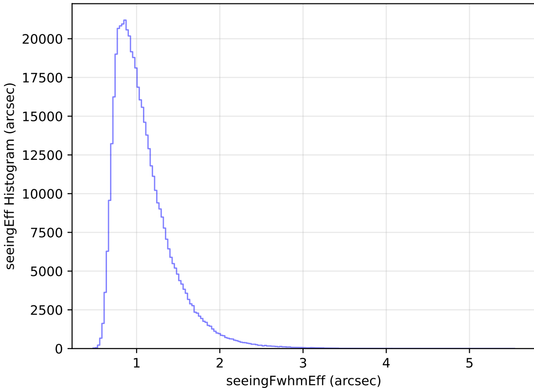
too_elab_heavy_r32_d2_griz_v3.4_10yrs All sky i band: seeingEff Histogram
