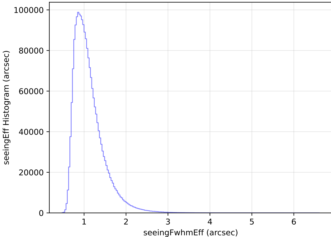
too_elab_heavy_r32_d2_griz_v3.4_10yrs All sky all bands: seeingEff Histogram
