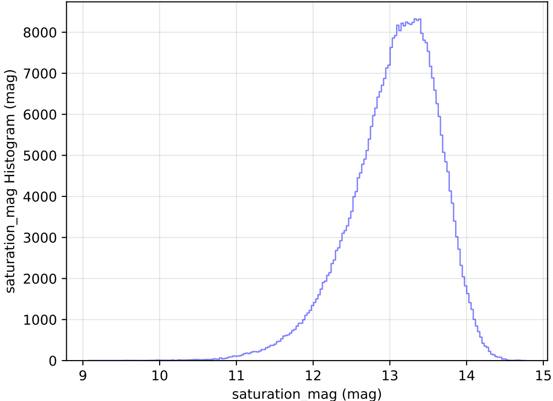
too_elab_heavy_r32_d2_griz_v3.4_10yrs WFD y band: saturation_mag Histogram
