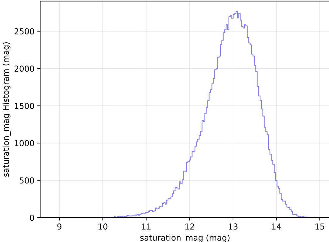
too_elab_heavy_r32_d2_griz_v3.4_10yrs WFD u band: saturation_mag Histogram
