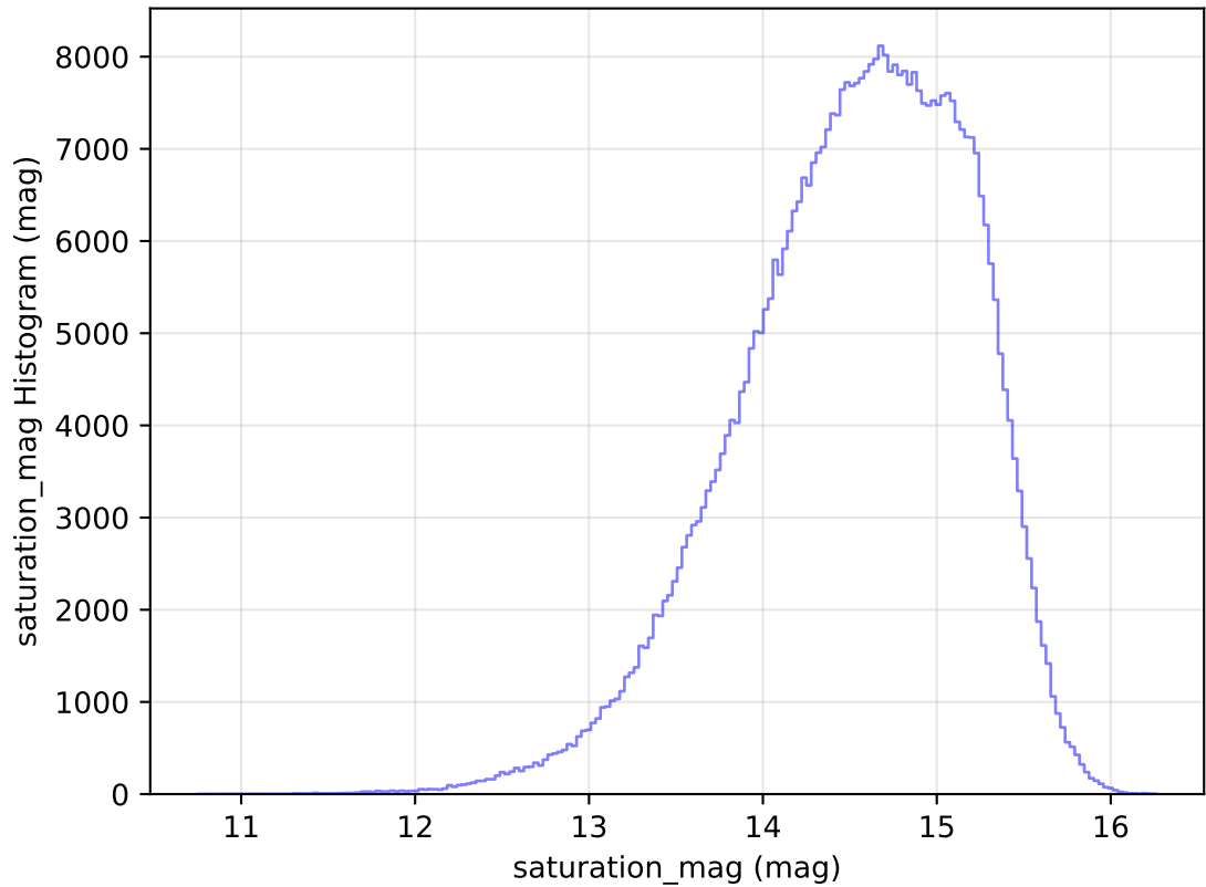
too_elab_heavy_r32_d2_griz_v3.4_10yrs WFD r band: saturation_mag Histogram
