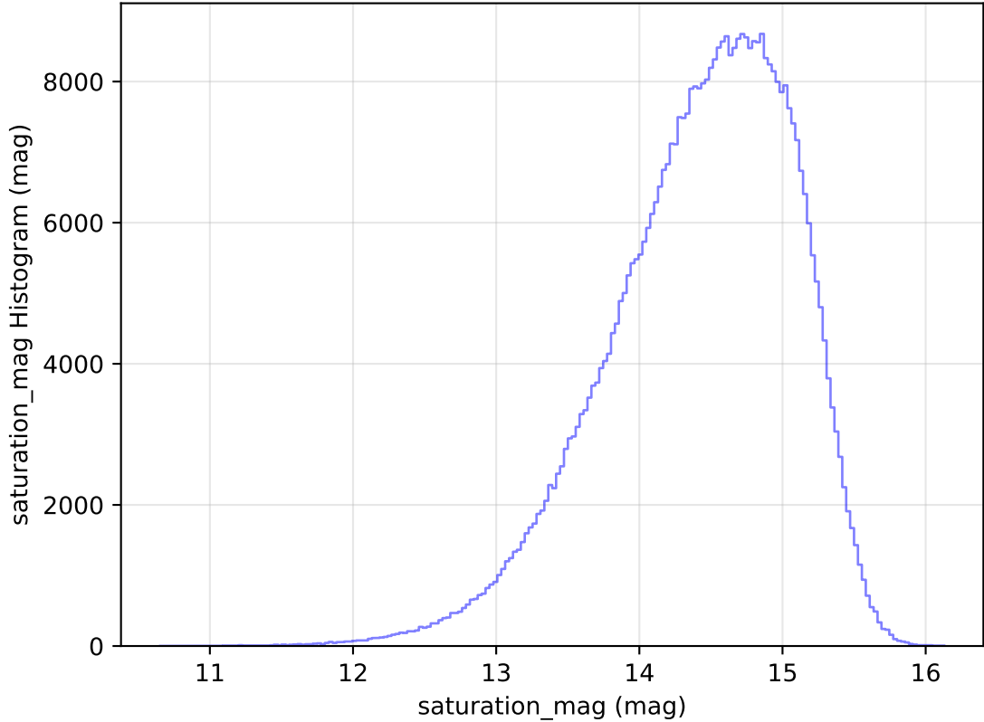
too_elab_heavy_r32_d2_griz_v3.4_10yrs WFD i band: saturation_mag Histogram
