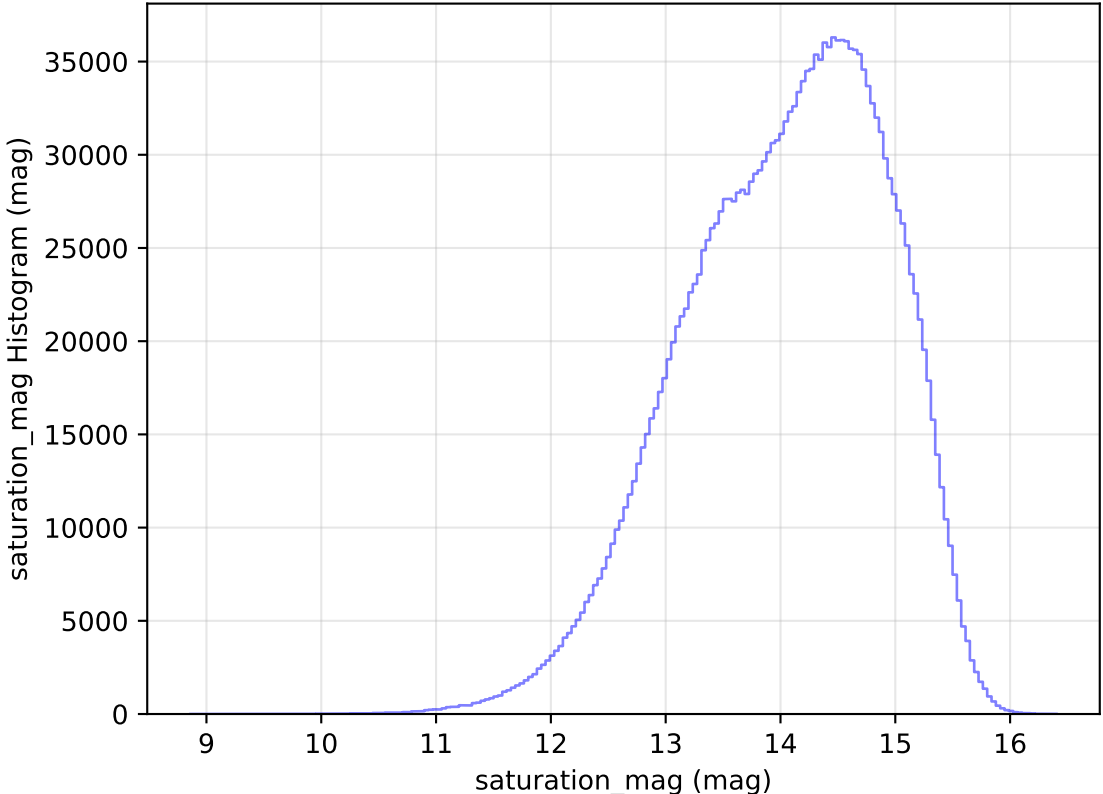
too_elab_heavy_r32_d2_griz_v3.4_10yrs WFD all bands: saturation_mag Histogram
