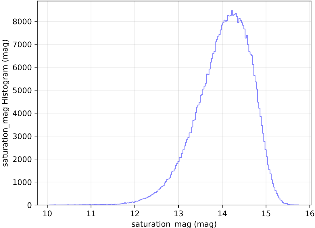
too_elab_heavy_r32_d2_griz_v3.4_10yrs All sky z band: saturation_mag Histogram
