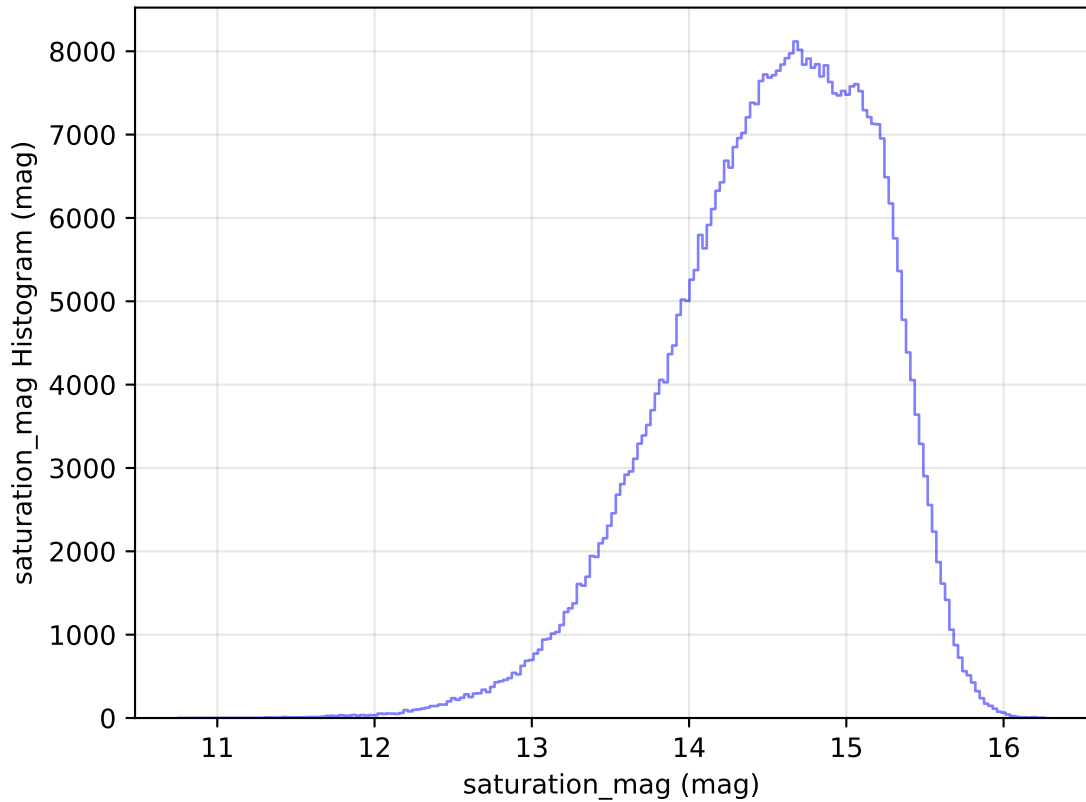
too_elab_heavy_r32_d2_griz_v3.4_10yrs All sky r band: saturation_mag Histogram
