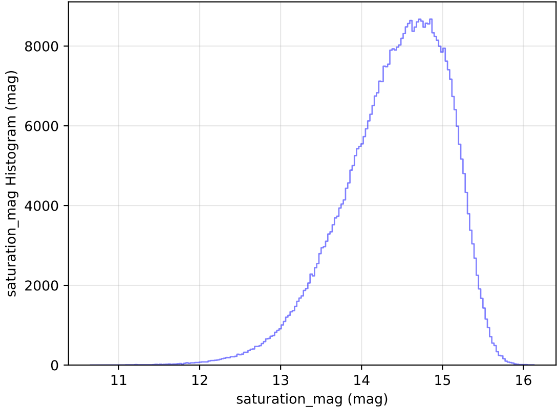
too_elab_heavy_r32_d2_griz_v3.4_10yrs All sky i band: saturation_mag Histogram
