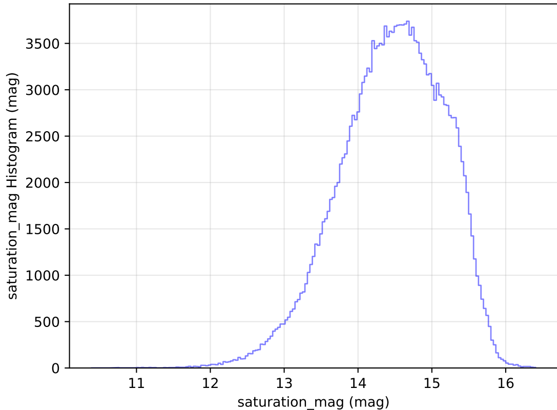
too_elab_heavy_r32_d2_griz_v3.4_10yrs All sky g band: saturation_mag Histogram
