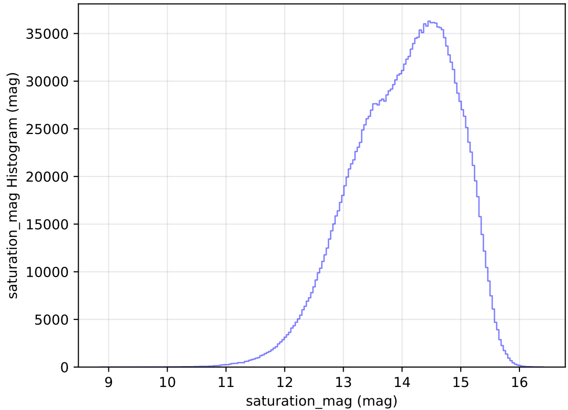
too_elab_heavy_r32_d2_griz_v3.4_10yrs All sky all bands: saturation_mag Histogram
