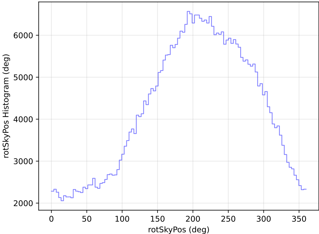
too_elab_heavy_r32_d2_griz_v3.4_10yrs WFD z band: rotSkyPos Histogram
