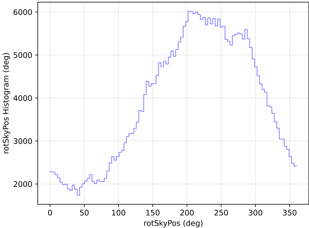
too_elab_heavy_r32_d2_griz_v3.4_10yrs WFD y band: rotSkyPos Histogram
