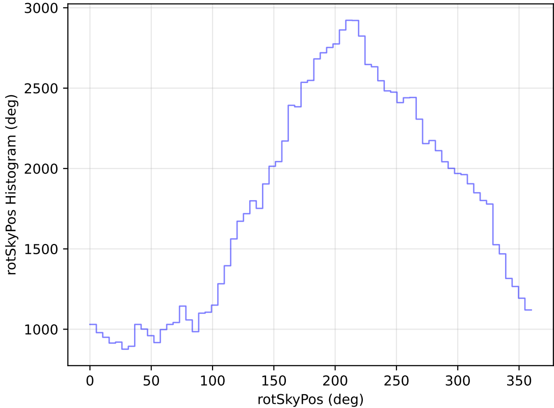
too_elab_heavy_r32_d2_griz_v3.4_10yrs WFD u band: rotSkyPos Histogram
