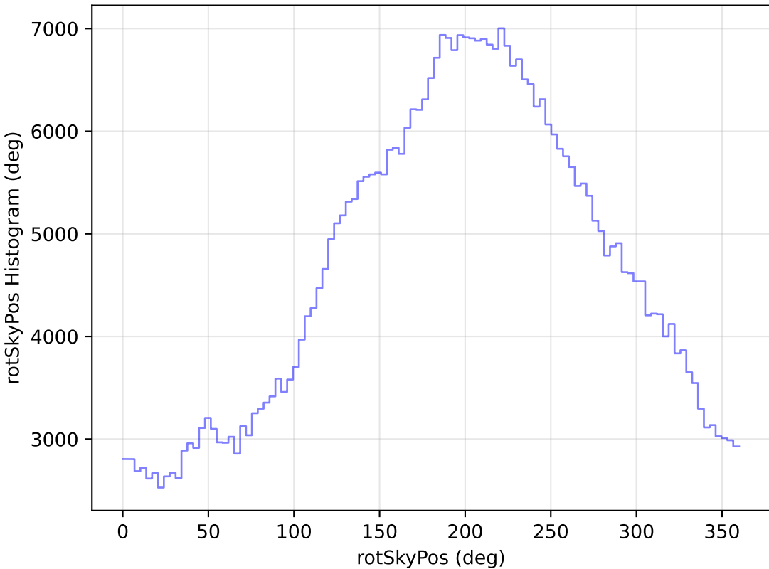
too_elab_heavy_r32_d2_griz_v3.4_10yrs WFD r band: rotSkyPos Histogram
