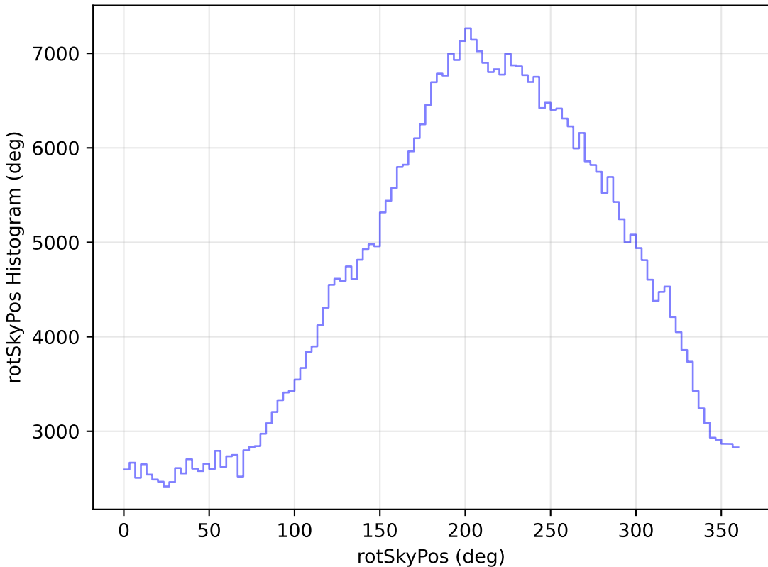
too_elab_heavy_r32_d2_griz_v3.4_10yrs WFD i band: rotSkyPos Histogram
