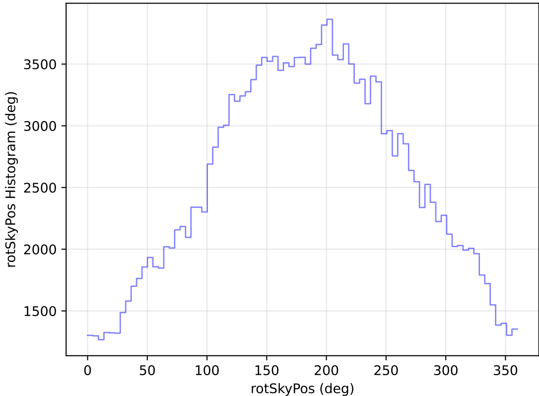
too_elab_heavy_r32_d2_griz_v3.4_10yrs WFD g band: rotSkyPos Histogram
