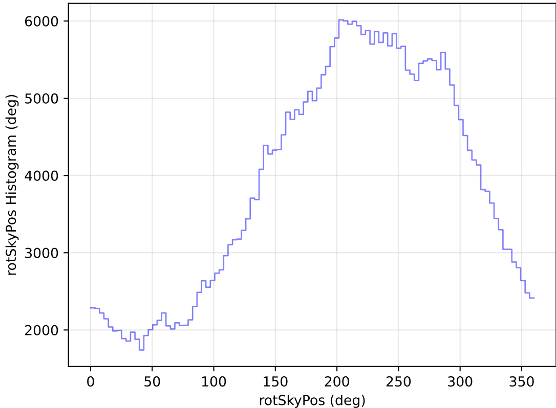
too_elab_heavy_r32_d2_griz_v3.4_10yrs All sky y band: rotSkyPos Histogram
