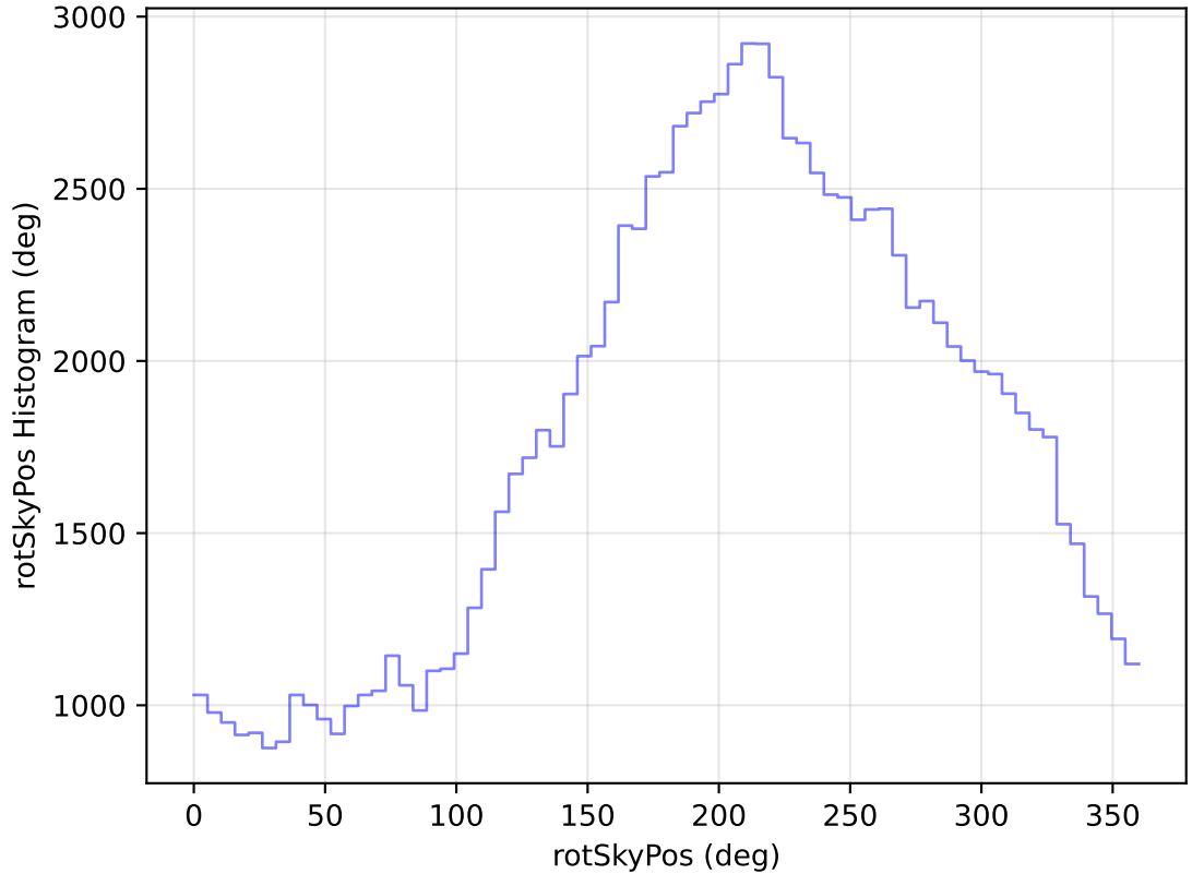
too_elab_heavy_r32_d2_griz_v3.4_10yrs All sky u band: rotSkyPos Histogram
