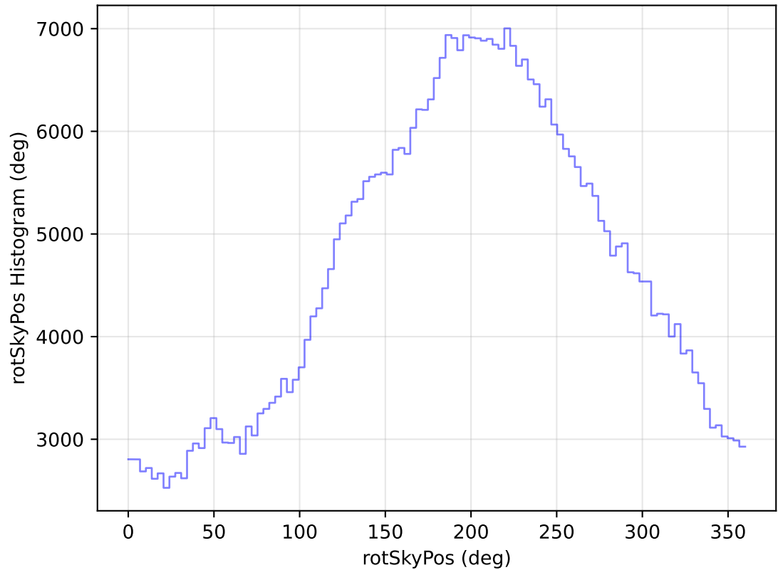
too_elab_heavy_r32_d2_griz_v3.4_10yrs All sky r band: rotSkyPos Histogram
