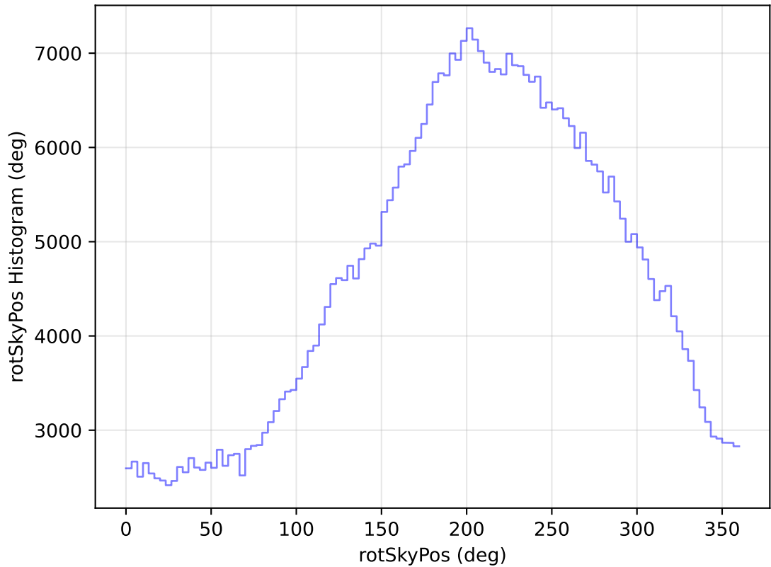
too_elab_heavy_r32_d2_griz_v3.4_10yrs All sky i band: rotSkyPos Histogram
