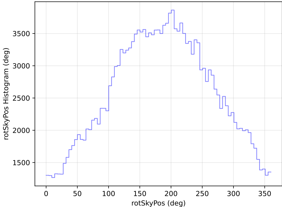
too_elab_heavy_r32_d2_griz_v3.4_10yrs All sky g band: rotSkyPos Histogram
