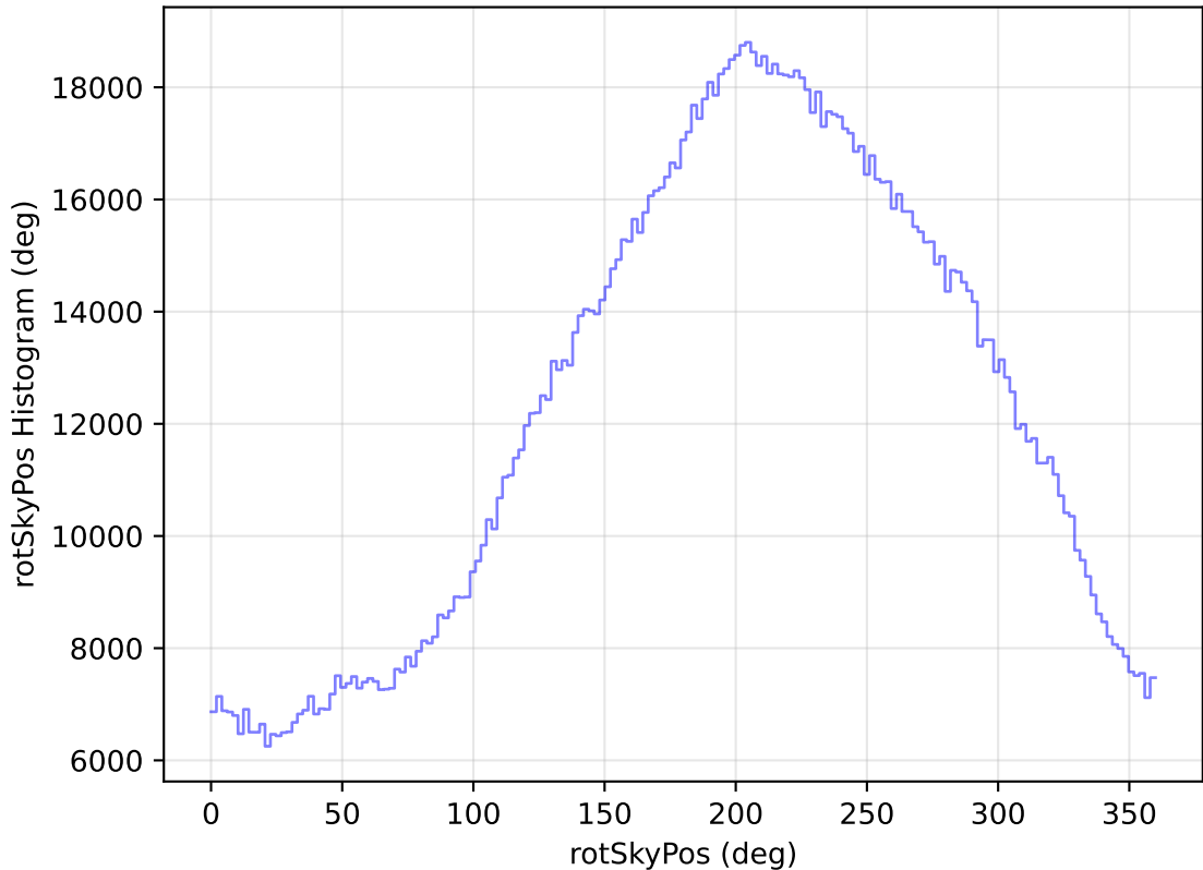
too_elab_heavy_r32_d2_griz_v3.4_10yrs All sky all bands: rotSkyPos Histogram
