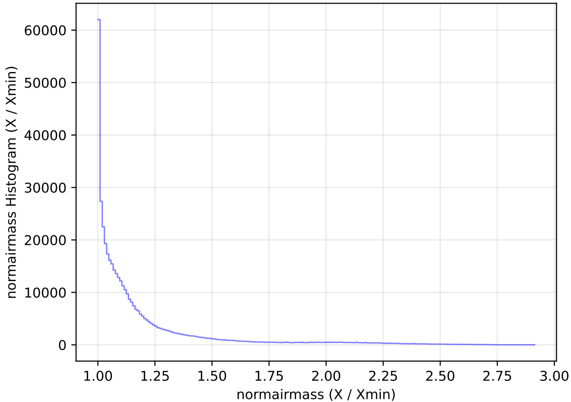
too_elab_heavy_r32_d2_griz_v3.4_10yrs WFD z band: normairmass Histogram
