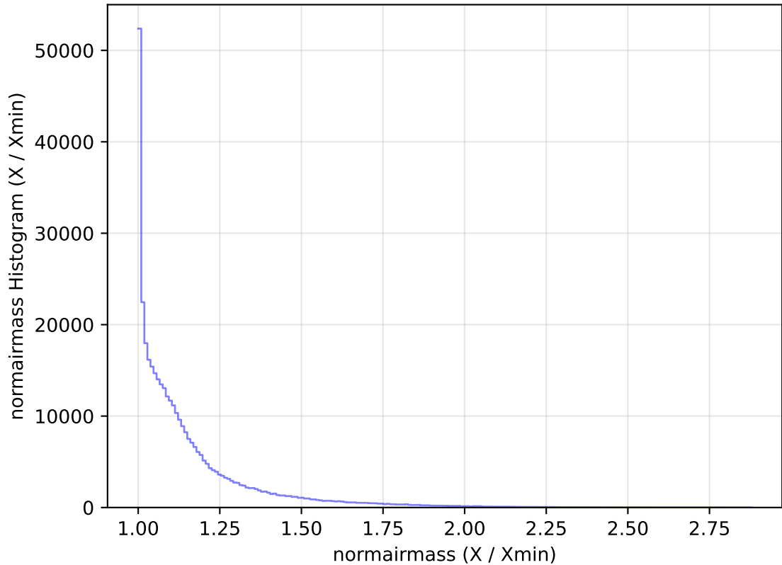
too_elab_heavy_r32_d2_griz_v3.4_10yrs WFD y band: normairmass Histogram
