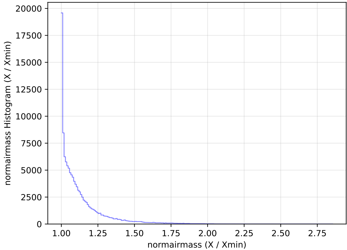
too_elab_heavy_r32_d2_griz_v3.4_10yrs WFD u band: normairmass Histogram
