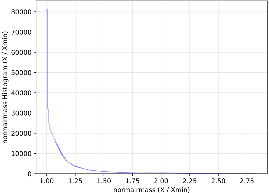
too_elab_heavy_r32_d2_griz_v3.4_10yrs WFD r band: normairmass Histogram
