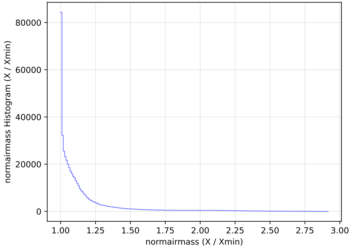
too_elab_heavy_r32_d2_griz_v3.4_10yrs WFD i band: normairmass Histogram
