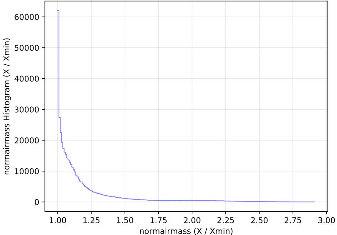
too_elab_heavy_r32_d2_griz_v3.4_10yrs All sky z band: normairmass Histogram
