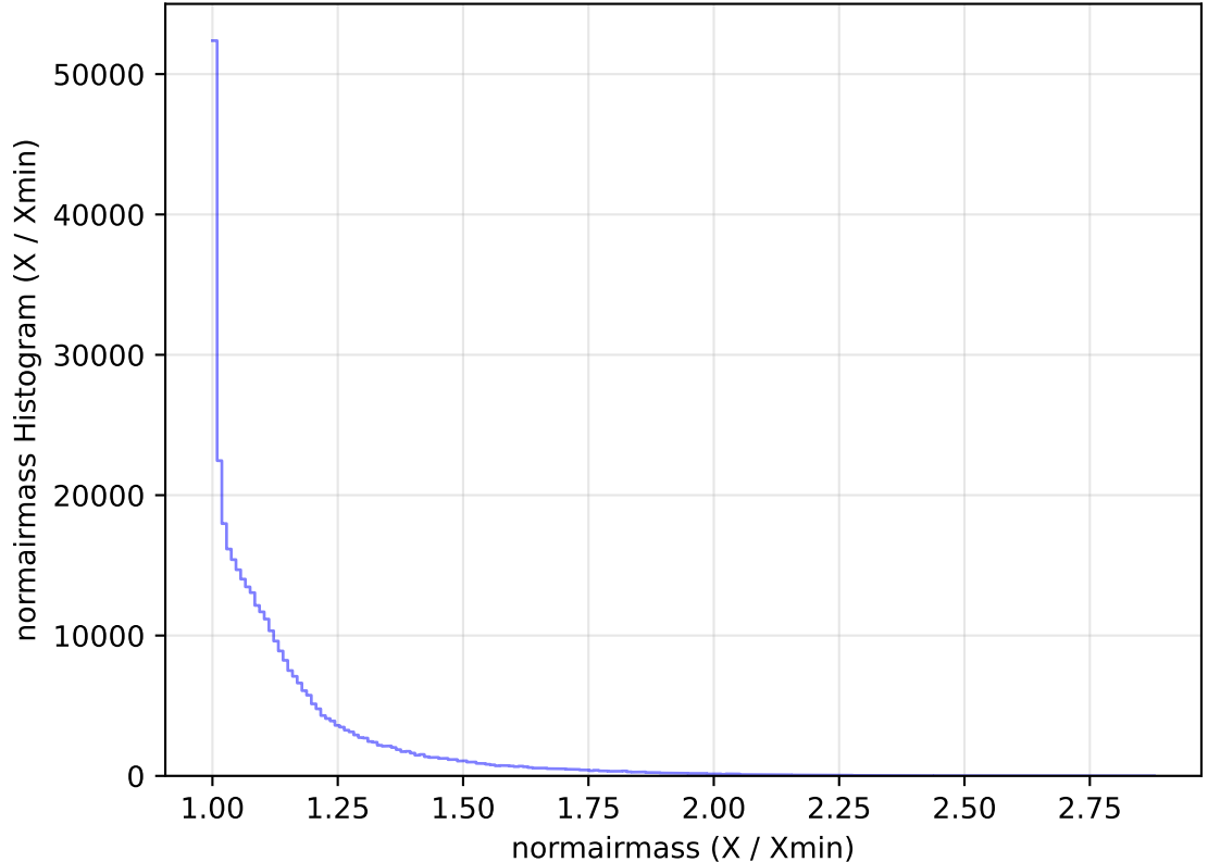
too_elab_heavy_r32_d2_griz_v3.4_10yrs All sky y band: normairmass Histogram
