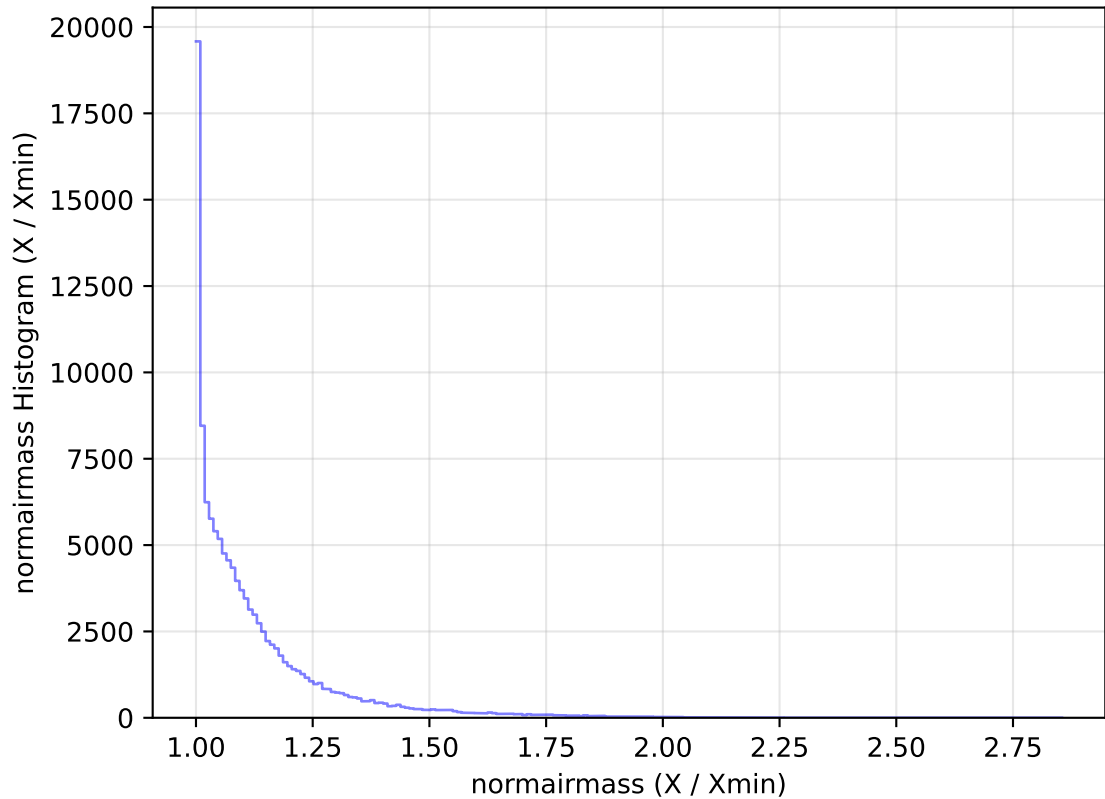
too_elab_heavy_r32_d2_griz_v3.4_10yrs All sky u band: normairmass Histogram
