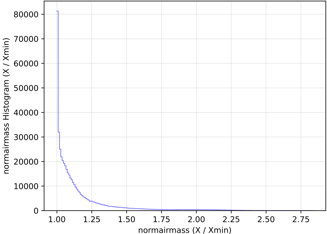
too_elab_heavy_r32_d2_griz_v3.4_10yrs All sky r band: normairmass Histogram
