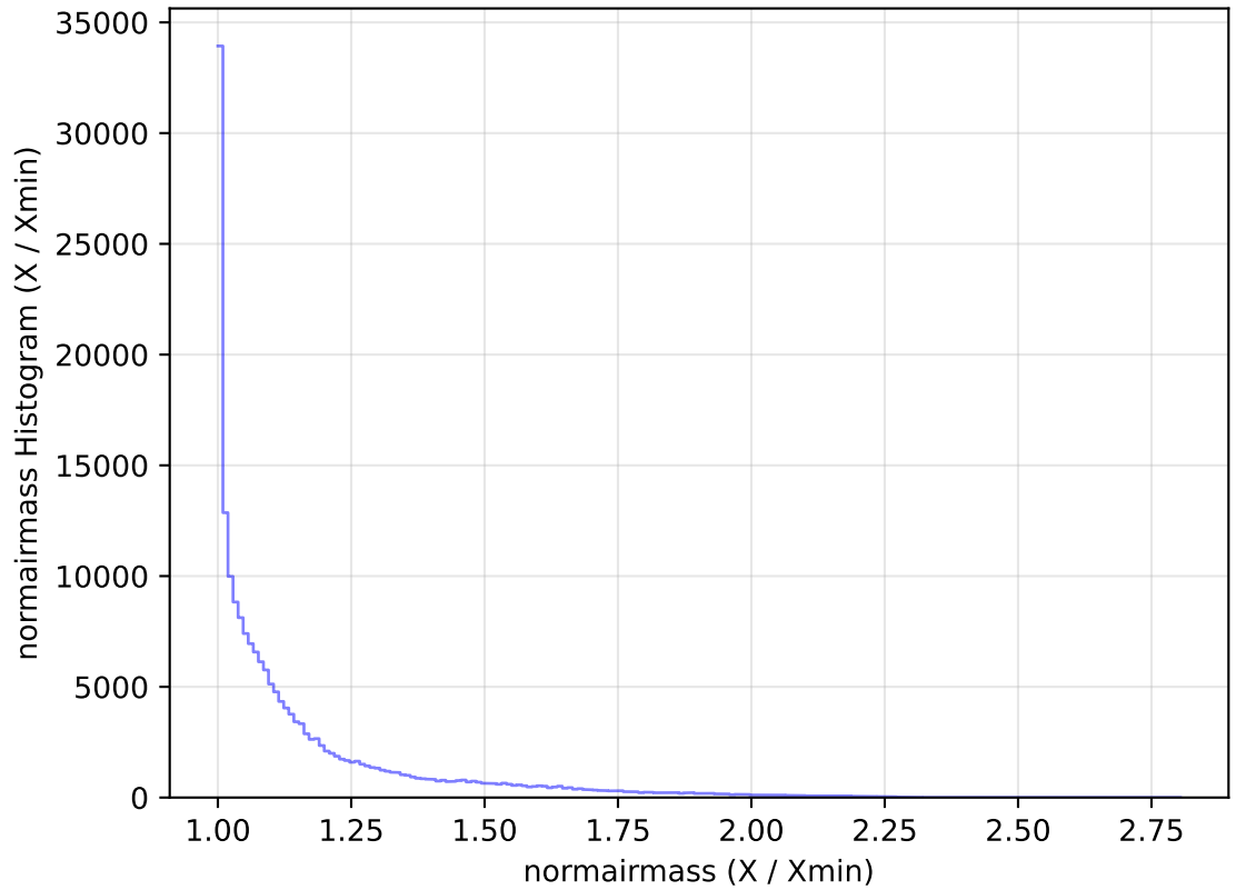
too_elab_heavy_r32_d2_griz_v3.4_10yrs All sky g band: normairmass Histogram
