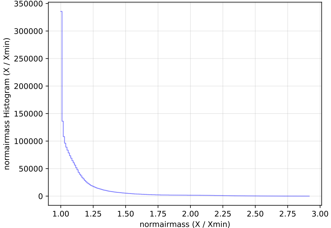
too_elab_heavy_r32_d2_griz_v3.4_10yrs All sky all bands: normairmass Histogram
