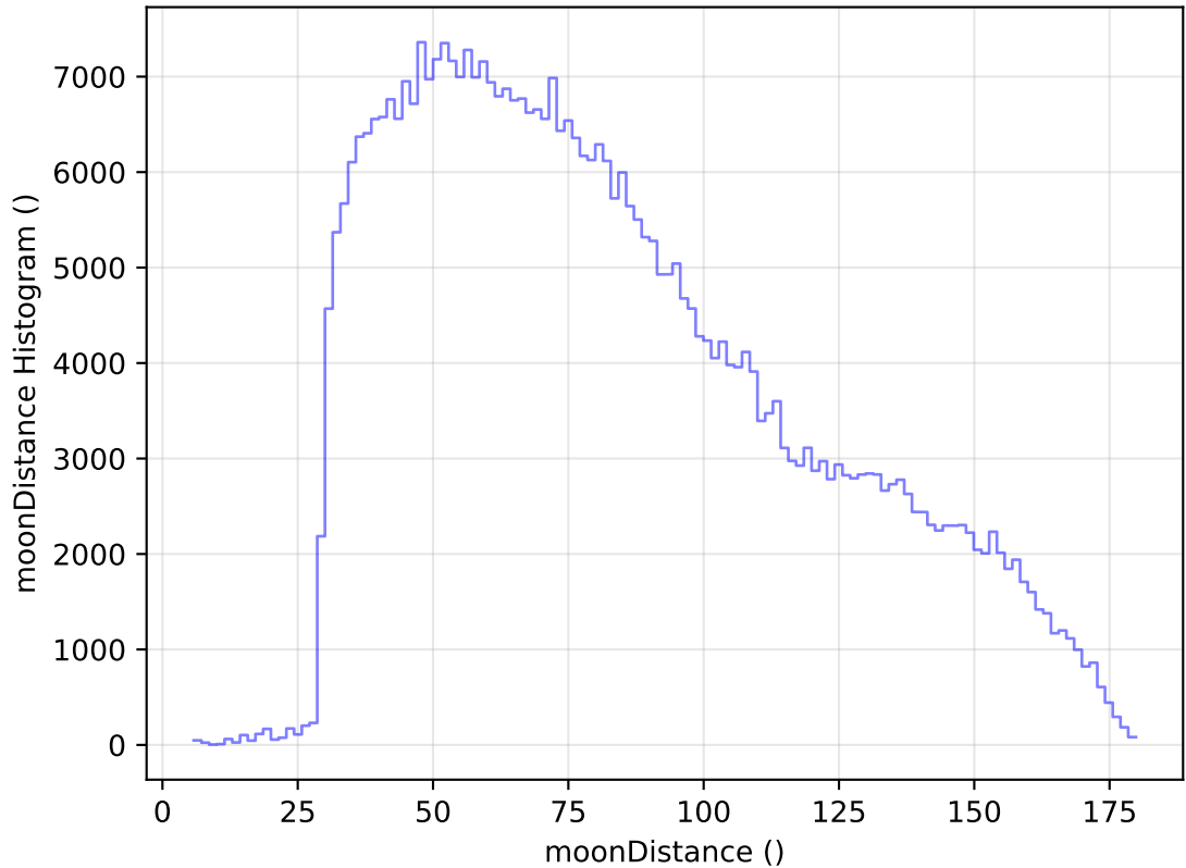
too_elab_heavy_r32_d2_griz_v3.4_10yrs WFD z band: moonDistance Histogram
