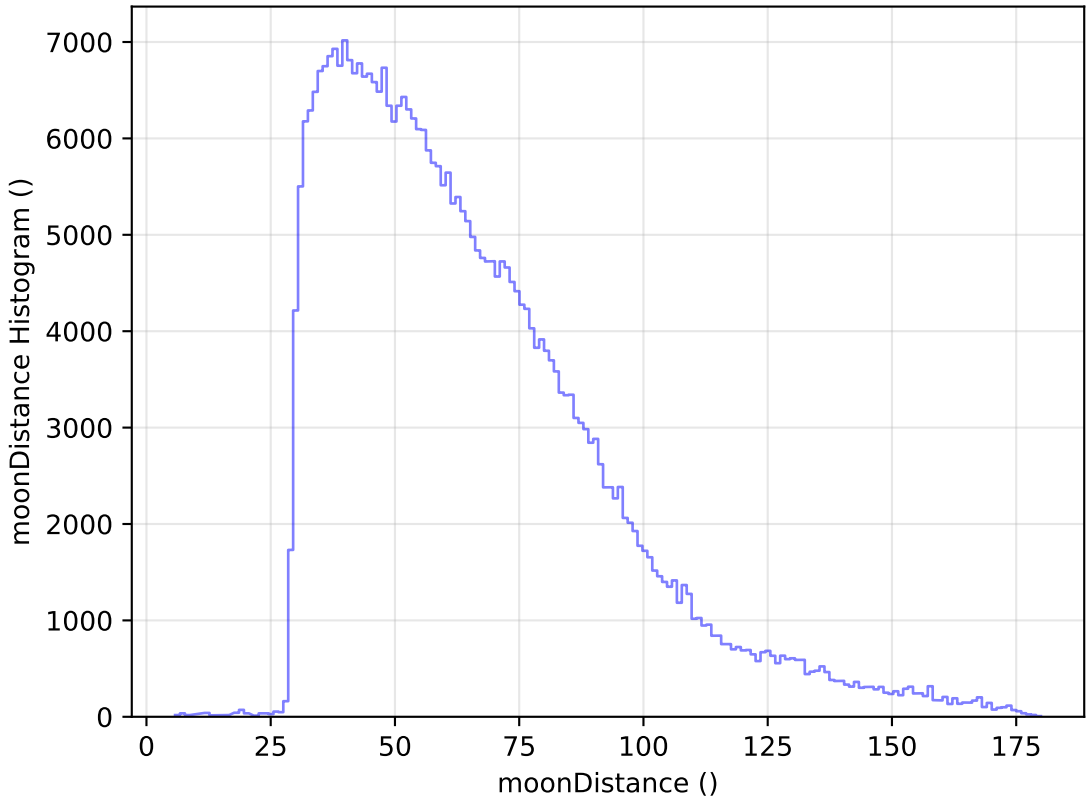
too_elab_heavy_r32_d2_griz_v3.4_10yrs WFD y band: moonDistance Histogram
