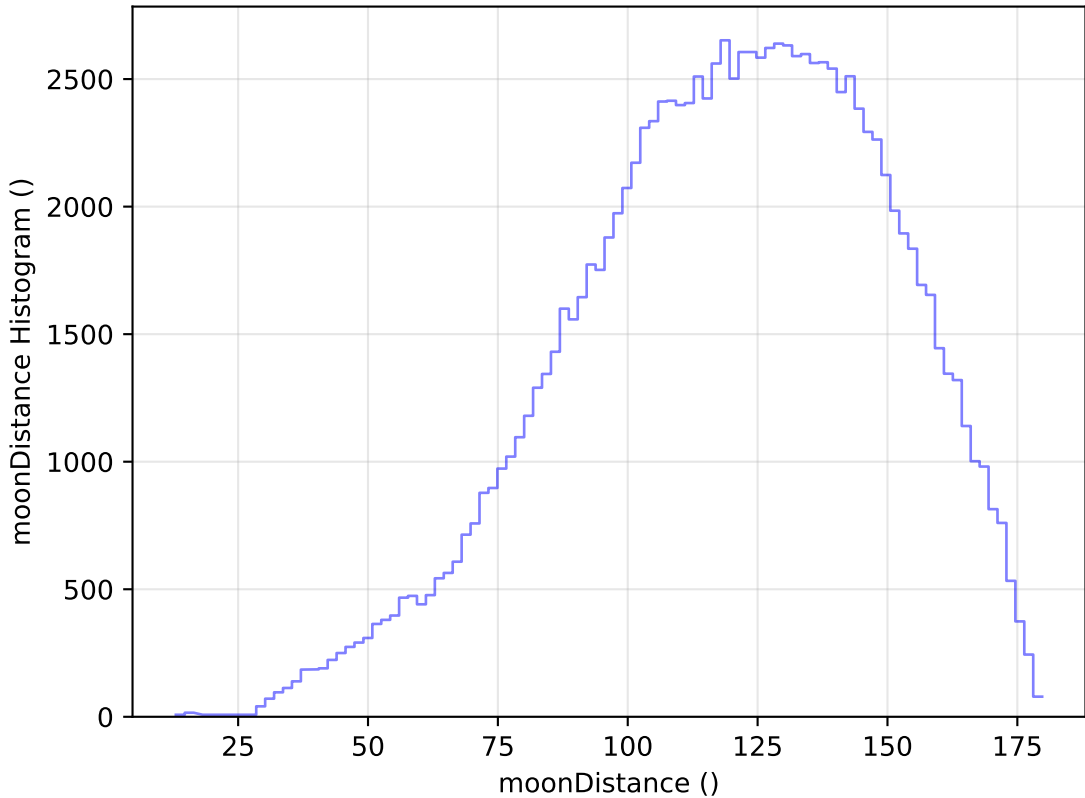
too_elab_heavy_r32_d2_griz_v3.4_10yrs WFD u band: moonDistance Histogram
