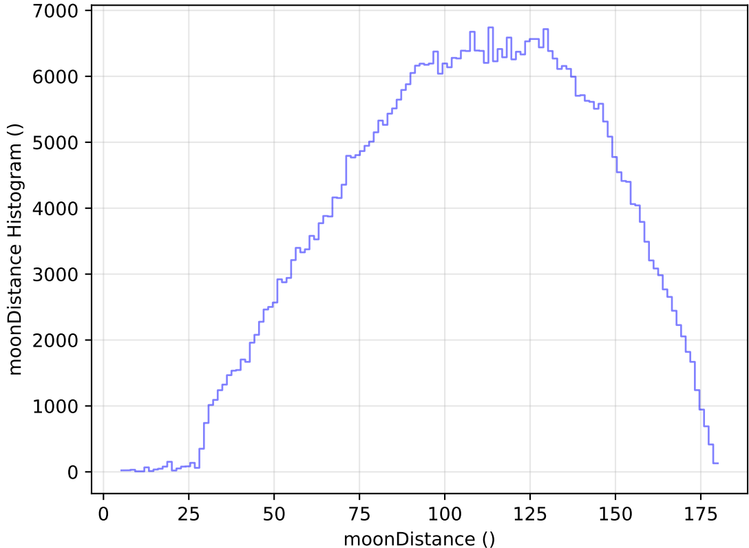
too_elab_heavy_r32_d2_griz_v3.4_10yrs WFD r band: moonDistance Histogram
