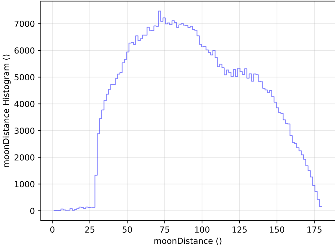
too_elab_heavy_r32_d2_griz_v3.4_10yrs WFD i band: moonDistance Histogram
