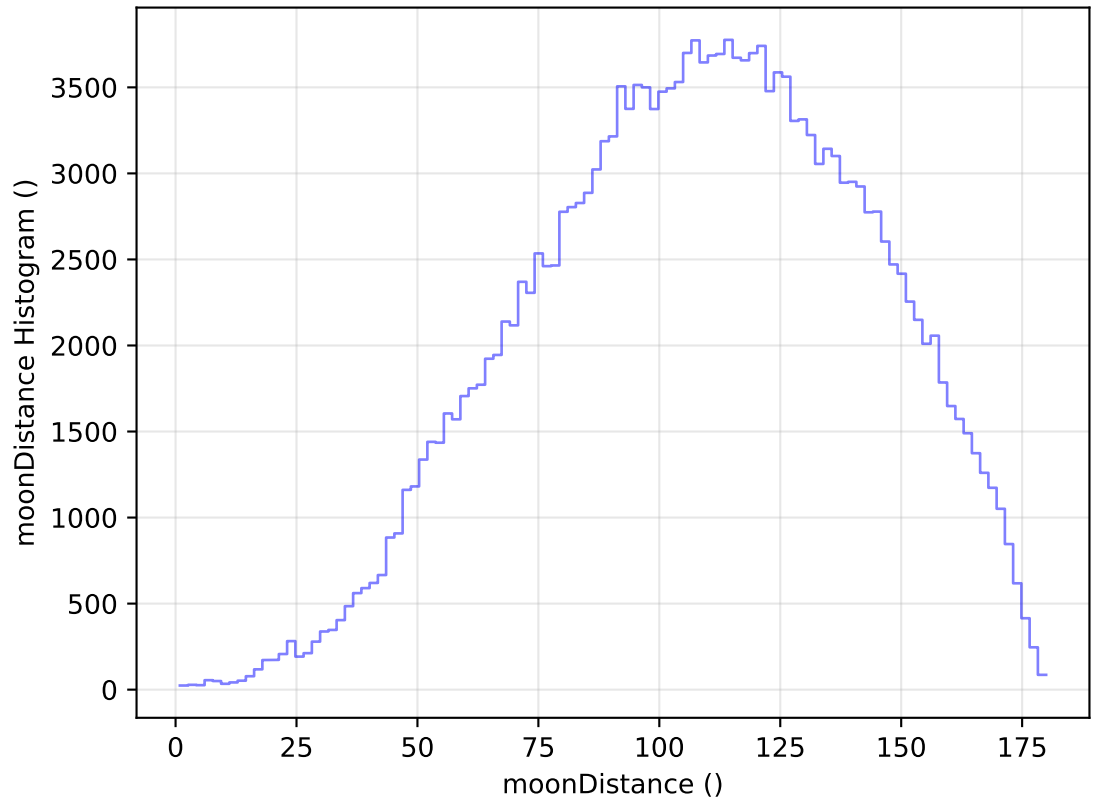
too_elab_heavy_r32_d2_griz_v3.4_10yrs WFD g band: moonDistance Histogram
