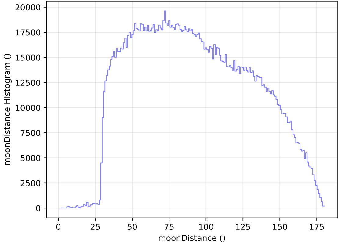
too_elab_heavy_r32_d2_griz_v3.4_10yrs WFD all bands: moonDistance Histogram
