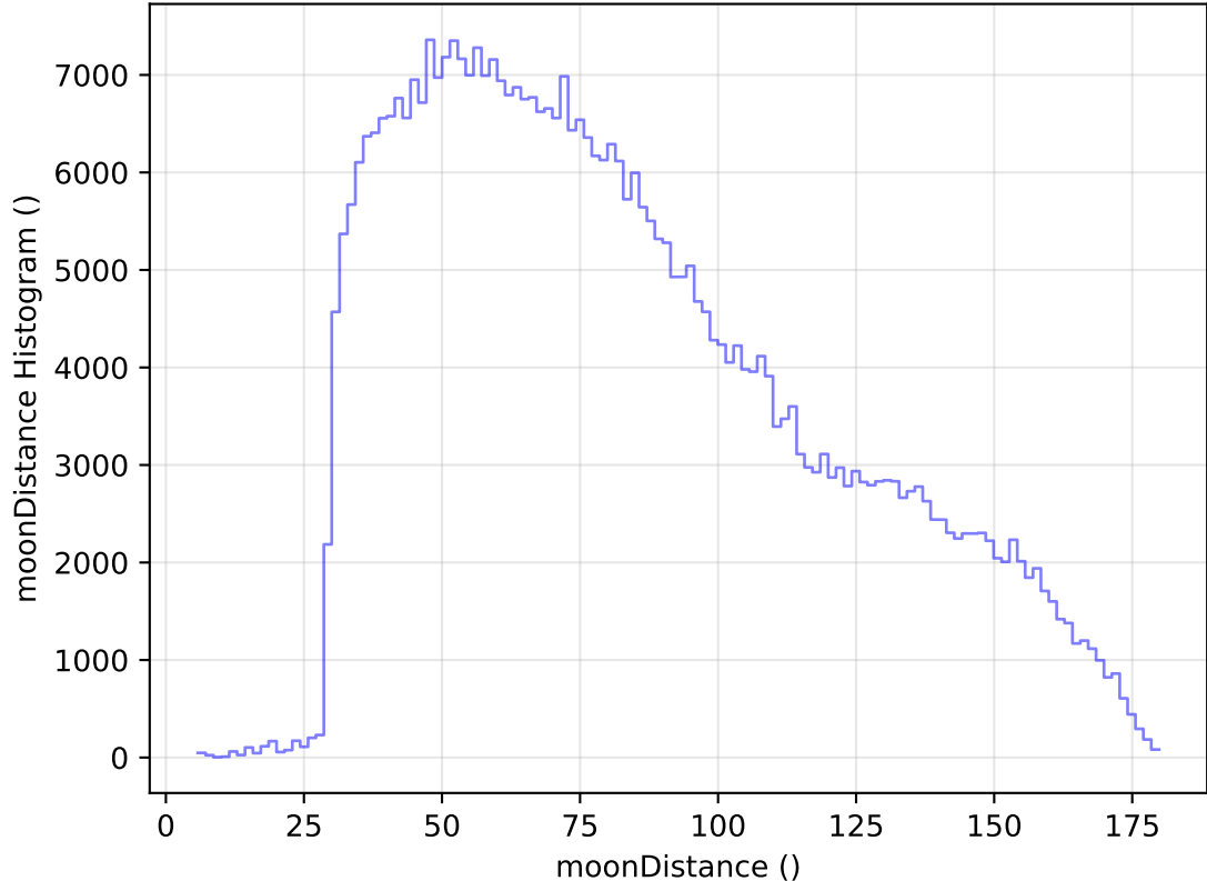
too_elab_heavy_r32_d2_griz_v3.4_10yrs All sky z band: moonDistance Histogram
