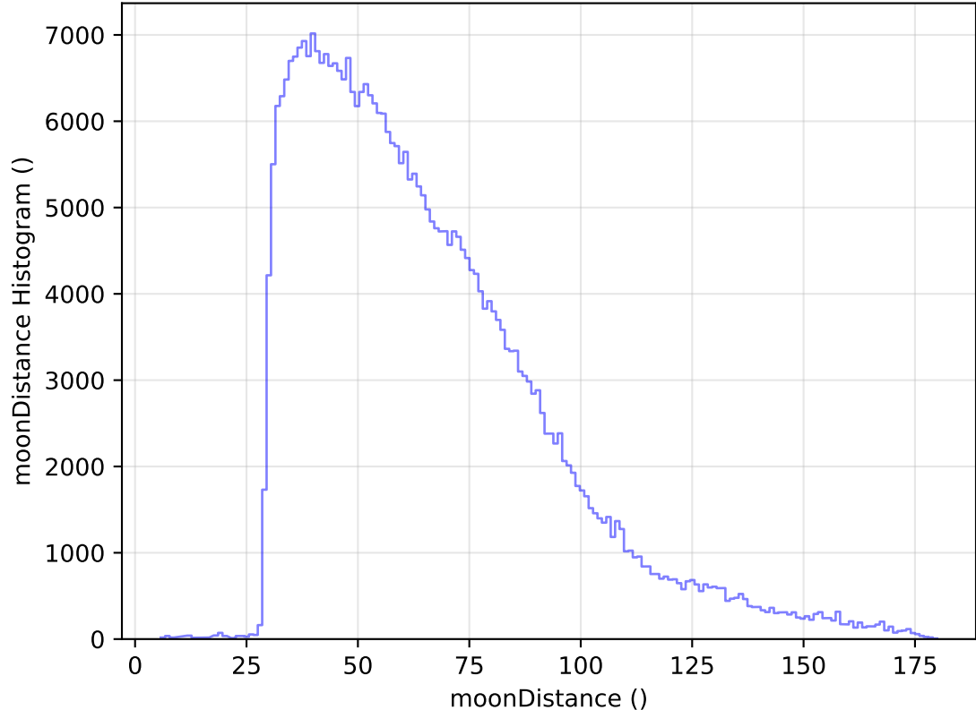
too_elab_heavy_r32_d2_griz_v3.4_10yrs All sky y band: moonDistance Histogram
