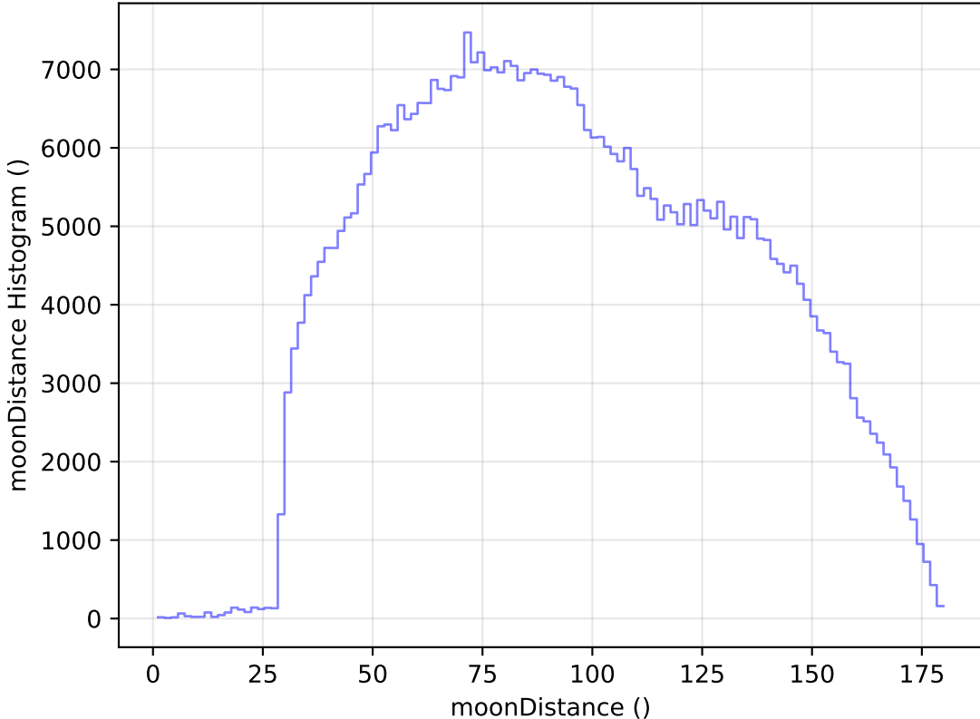
too_elab_heavy_r32_d2_griz_v3.4_10yrs All sky i band: moonDistance Histogram
