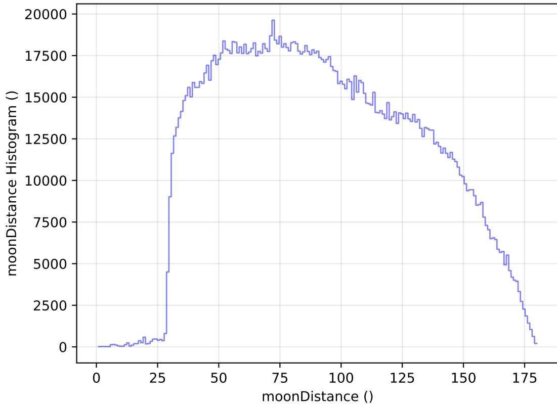
too_elab_heavy_r32_d2_griz_v3.4_10yrs All sky all bands: moonDistance Histogram
