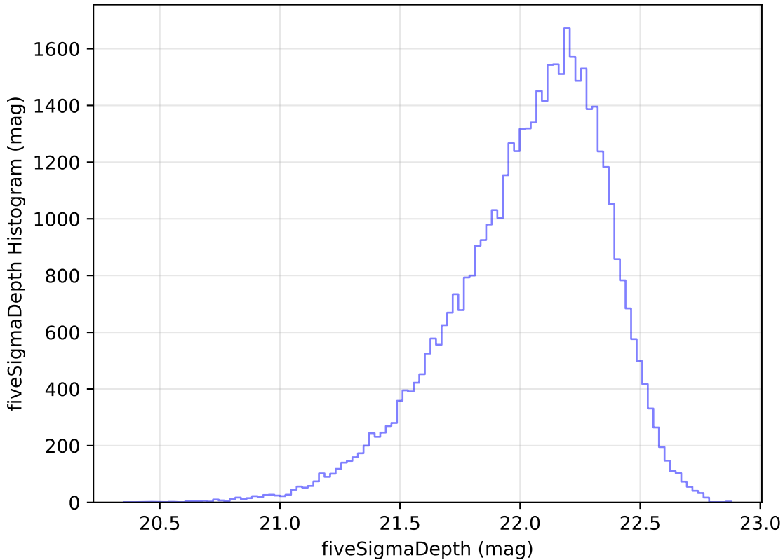
too_elab_heavy_r32_d2_griz_v3.4_10yrs Yr 1 y band: fiveSigmaDepth Histogram
